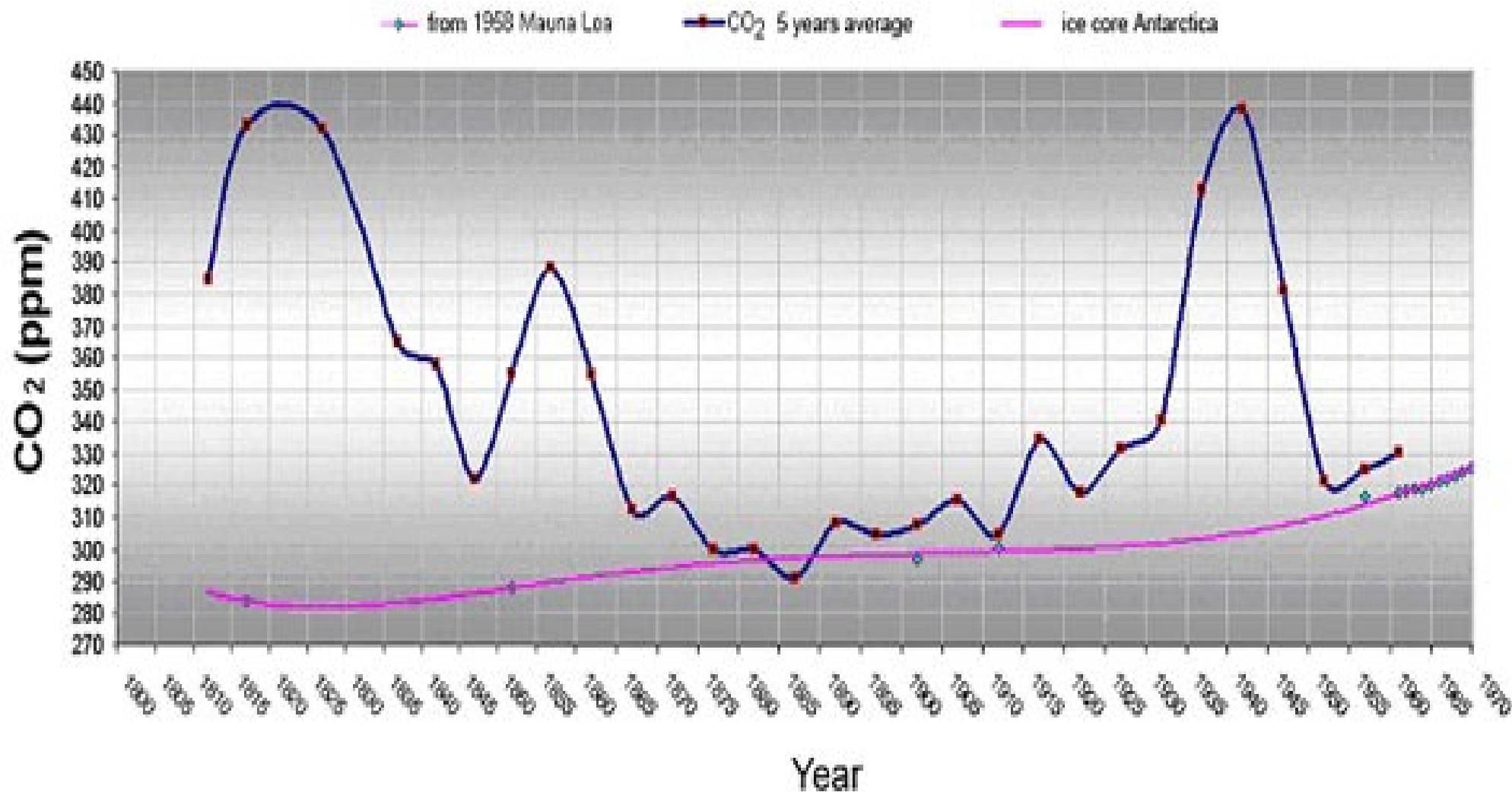
CO 2 -1812 - 2004 Northern Hemisphere , Chemical Measurement
